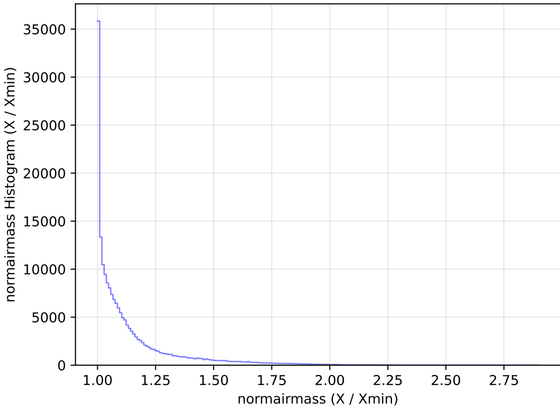
roll_pause_mjdp0_v3.4_10yrs All sky g band: normairmass Histogram
