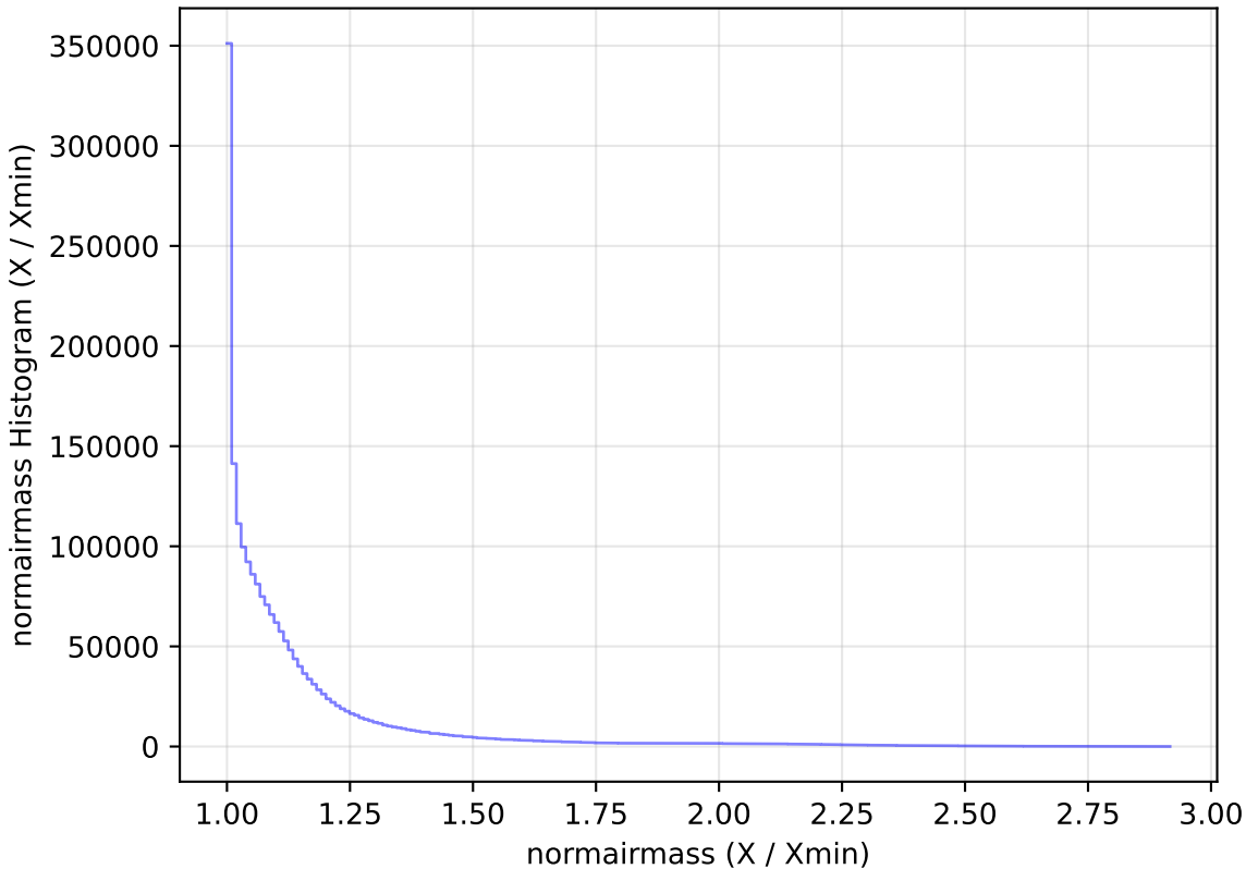
roll_pause_mjdp0_v3.4_10yrs All sky all bands: normairmass Histogram
