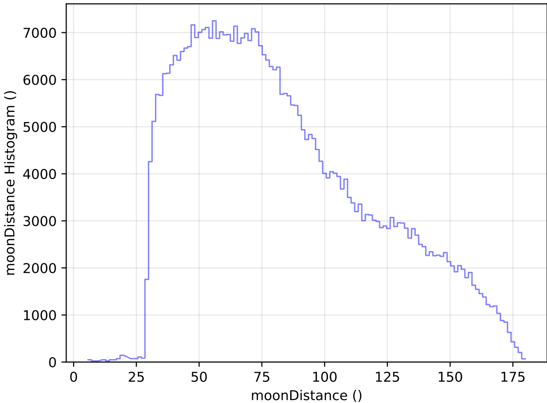
roll_pause_mjdp0_v3.4_10yrs WFD z band: moonDistance Histogram
