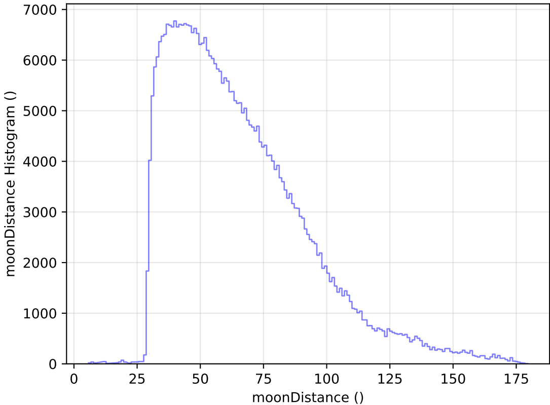
roll_pause_mjdp0_v3.4_10yrs WFD y band: moonDistance Histogram
