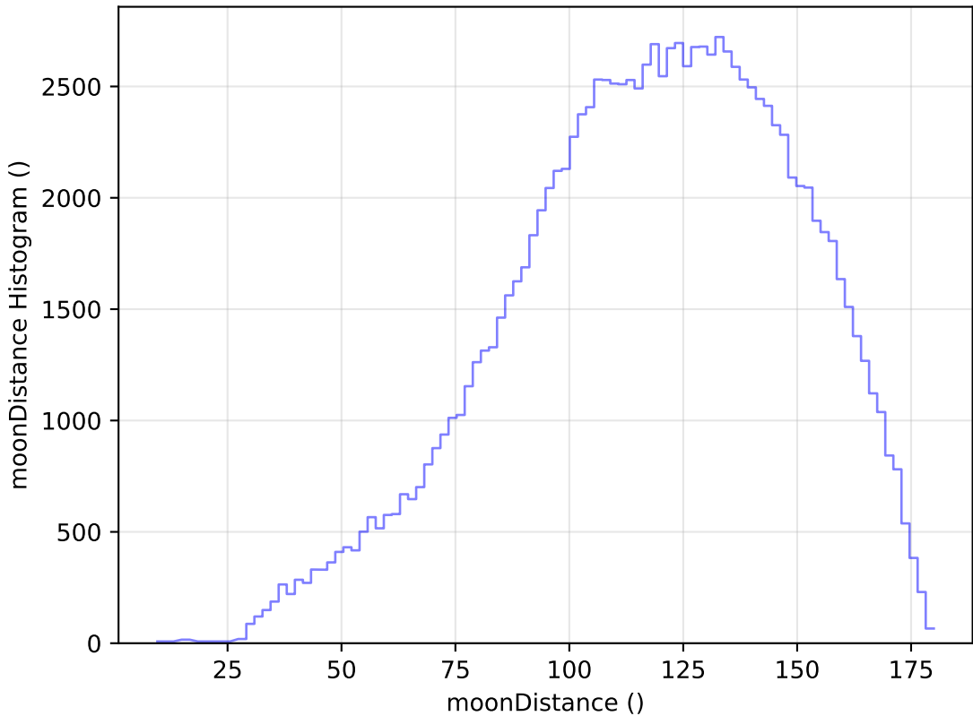
roll_pause_mjdp0_v3.4_10yrs WFD u band: moonDistance Histogram
