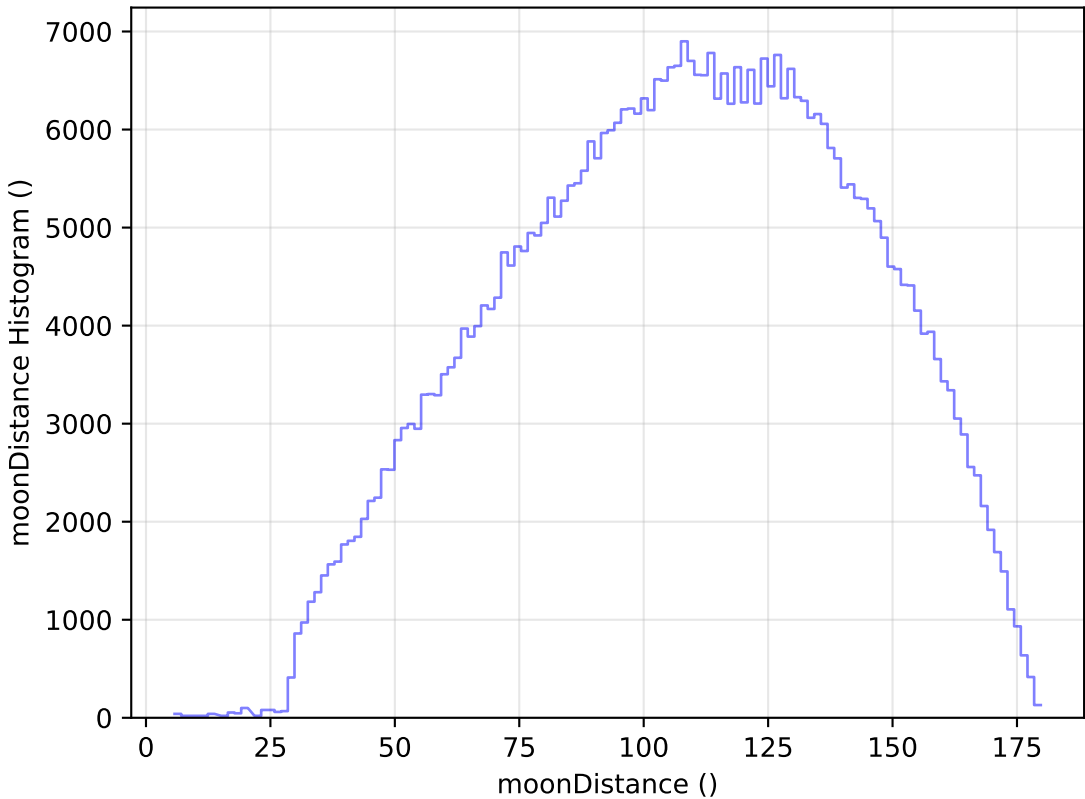
roll_pause_mjdp0_v3.4_10yrs WFD r band: moonDistance Histogram
