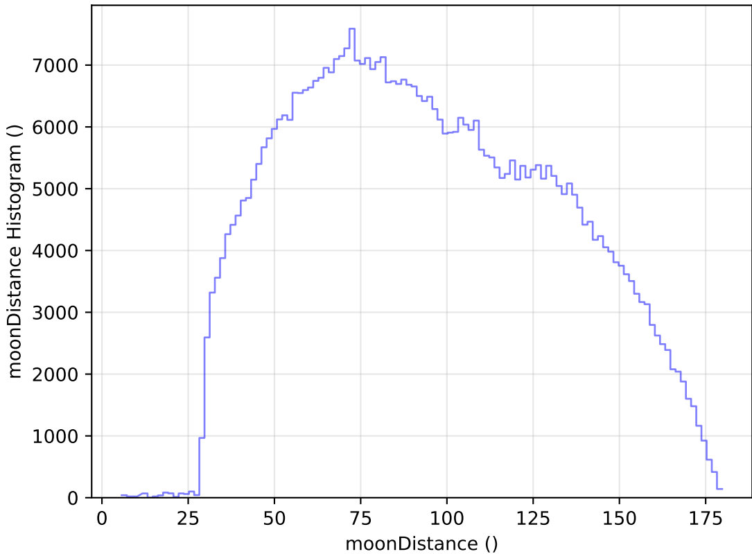
roll_pause_mjdp0_v3.4_10yrs WFD i band: moonDistance Histogram
