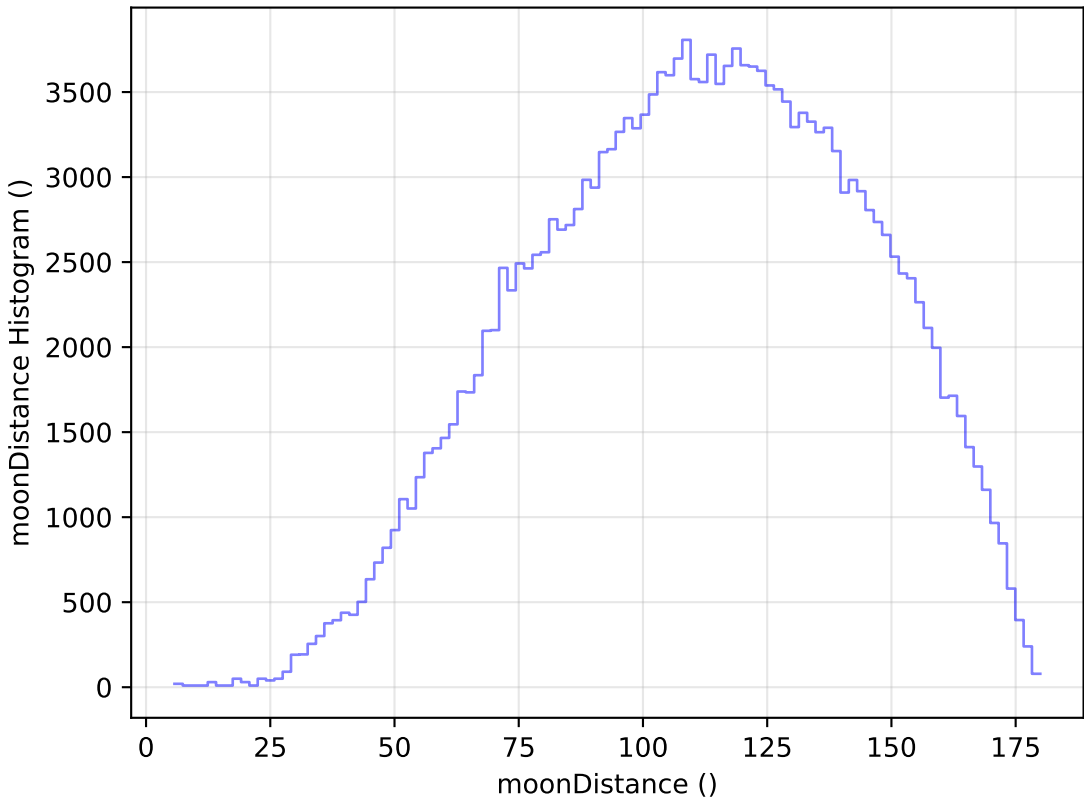
roll_pause_mjdp0_v3.4_10yrs WFD g band: moonDistance Histogram
