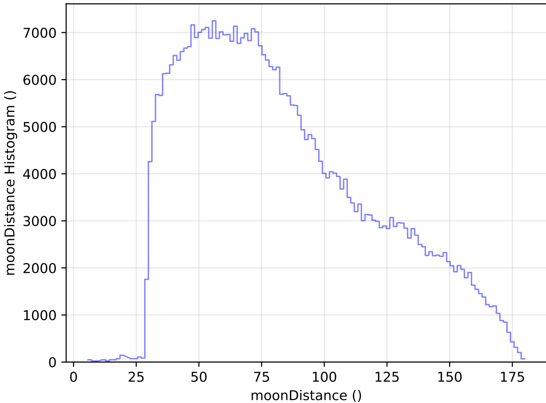
roll_pause_mjdp0_v3.4_10yrs All sky z band: moonDistance Histogram
