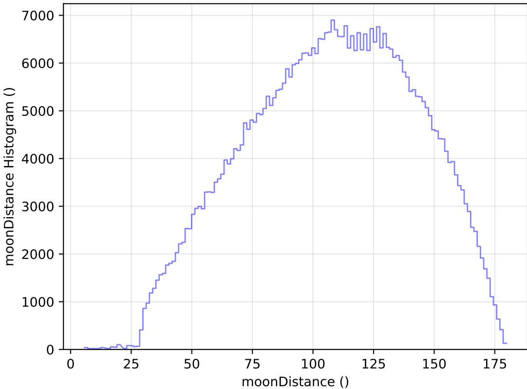
roll_pause_mjdp0_v3.4_10yrs All sky r band: moonDistance Histogram
