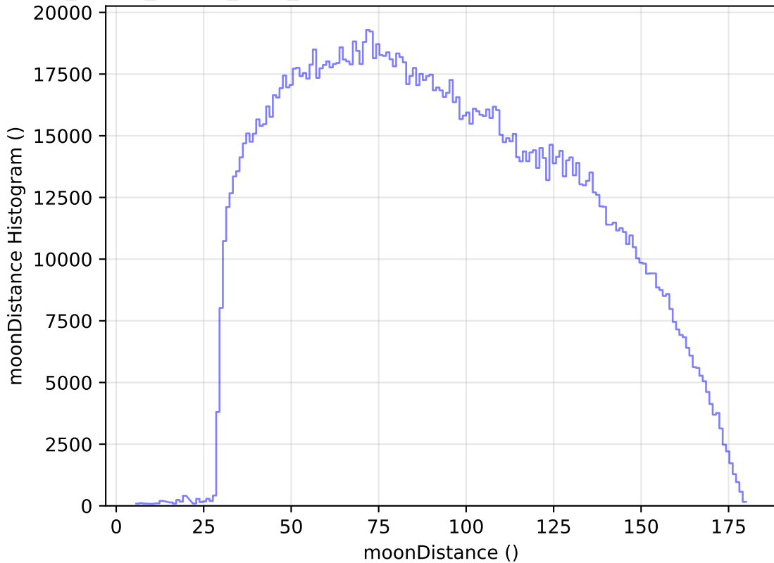
roll_pause_mjdp0_v3.4_10yrs All sky all bands: moonDistance Histogram
