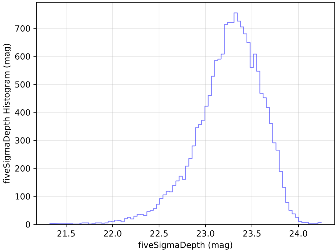
roll_pause_mjdp0_v3.4_10yrs Yr 1 u band: fiveSigmaDepth Histogram
