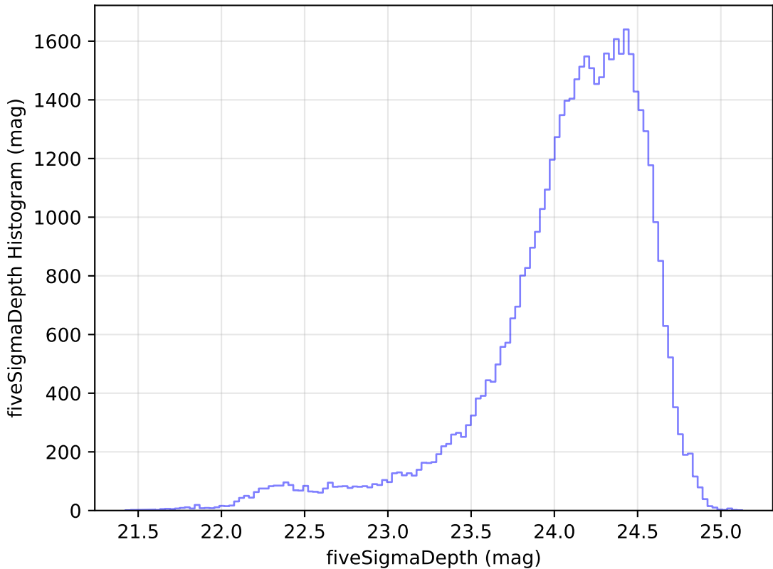
roll_pause_mjdp0_v3.4_10yrs Yr 1 r band: fiveSigmaDepth Histogram
