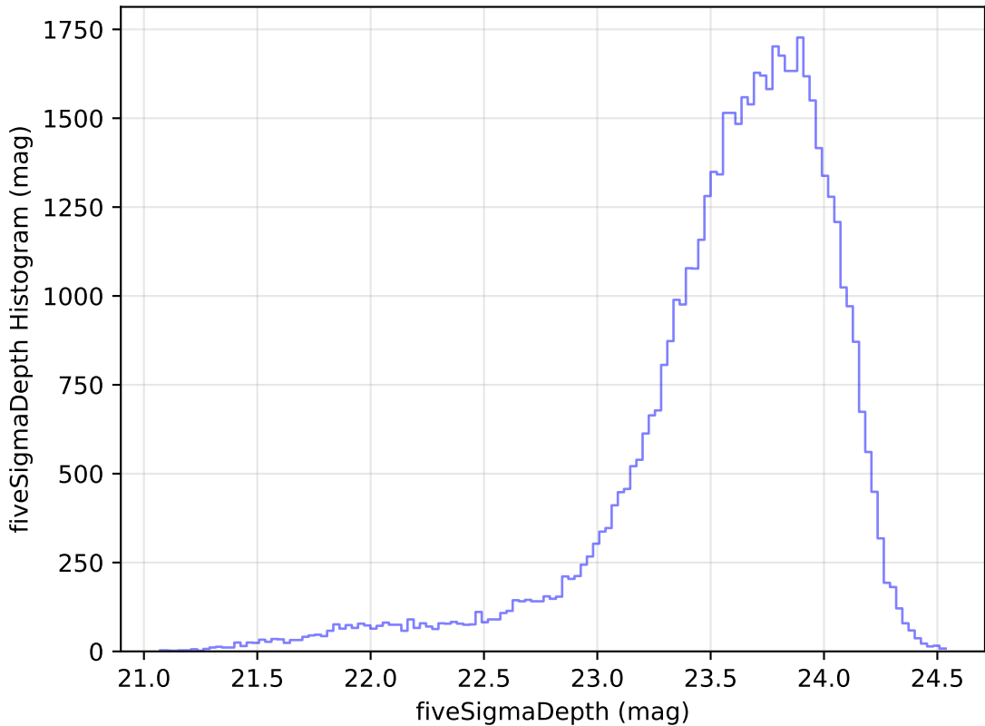
roll_pause_mjdp0_v3.4_10yrs Yr 1 i band: fiveSigmaDepth Histogram
