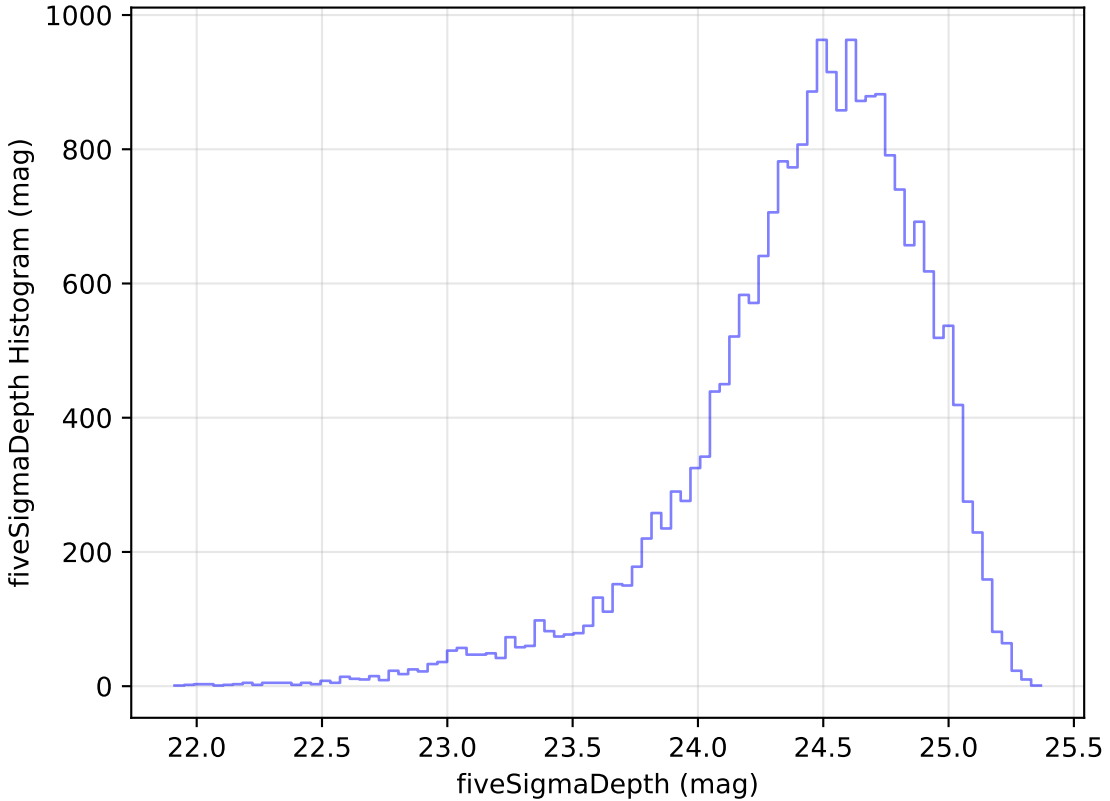
roll_pause_mjdp0_v3.4_10yrs Yr 1 g band: fiveSigmaDepth Histogram
