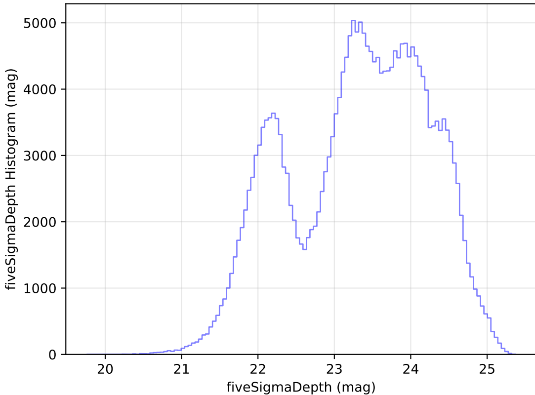
roll_pause_mjdp0_v3.4_10yrs Yr 1 all bands: fiveSigmaDepth Histogram
