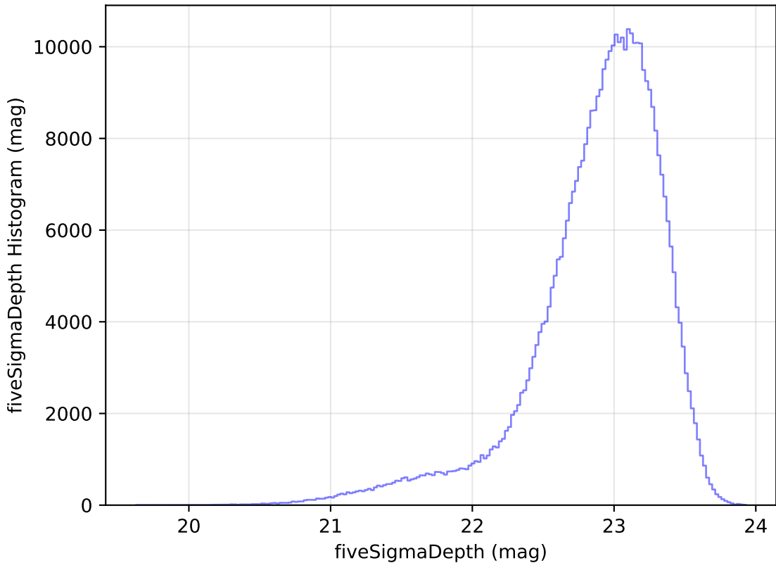
roll_pause_mjdp0_v3.4_10yrs WFD z band: fiveSigmaDepth Histogram
