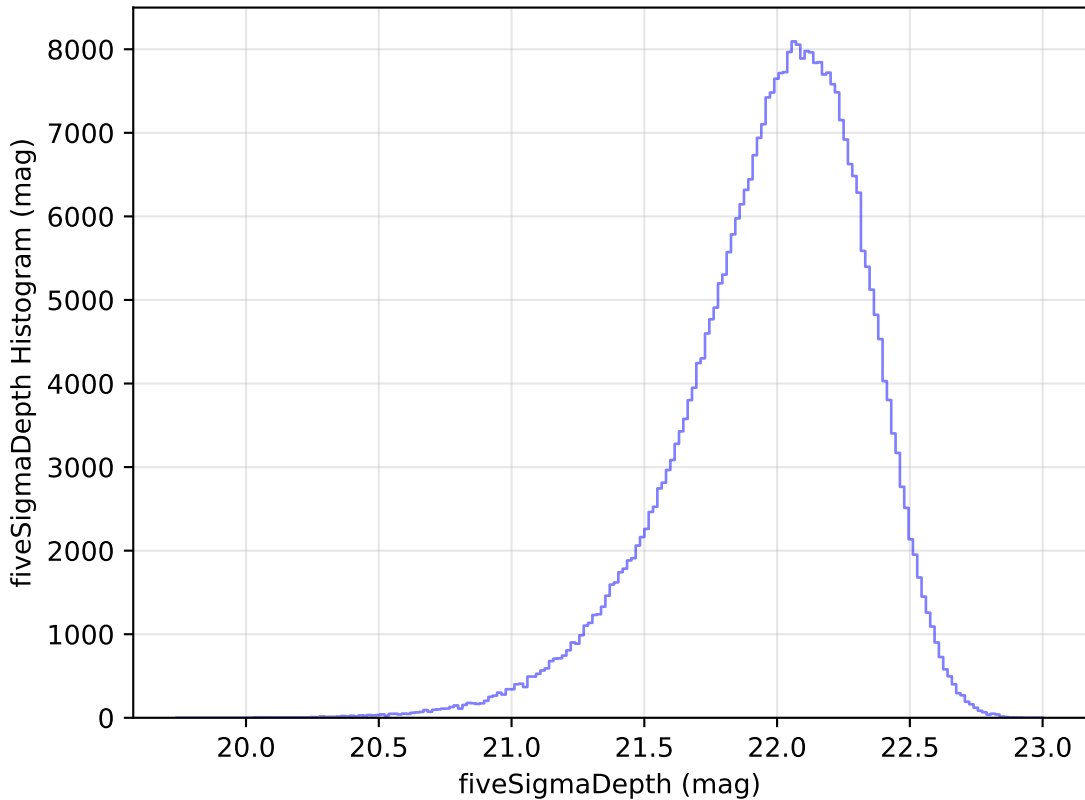
roll_pause_mjdp0_v3.4_10yrs WFD y band: fiveSigmaDepth Histogram
