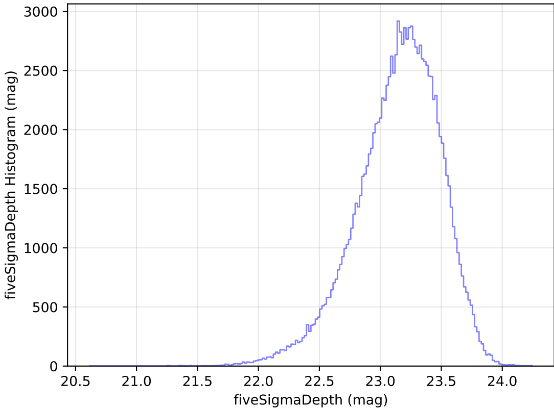
roll_pause_mjdp0_v3.4_10yrs WFD u band: fiveSigmaDepth Histogram
