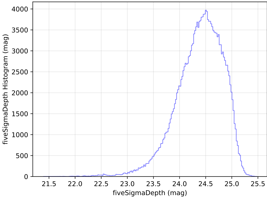
roll_pause_mjdp0_v3.4_10yrs WFD g band: fiveSigmaDepth Histogram
