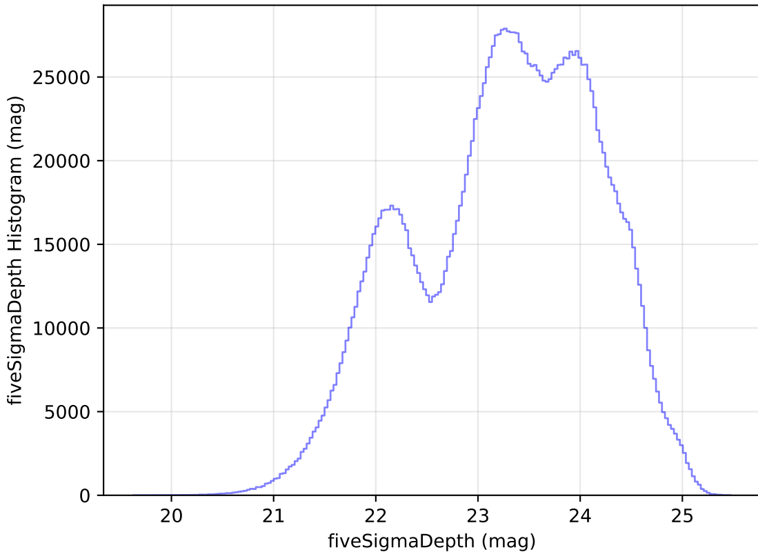
roll_pause_mjdp0_v3.4_10yrs WFD all bands: fiveSigmaDepth Histogram
