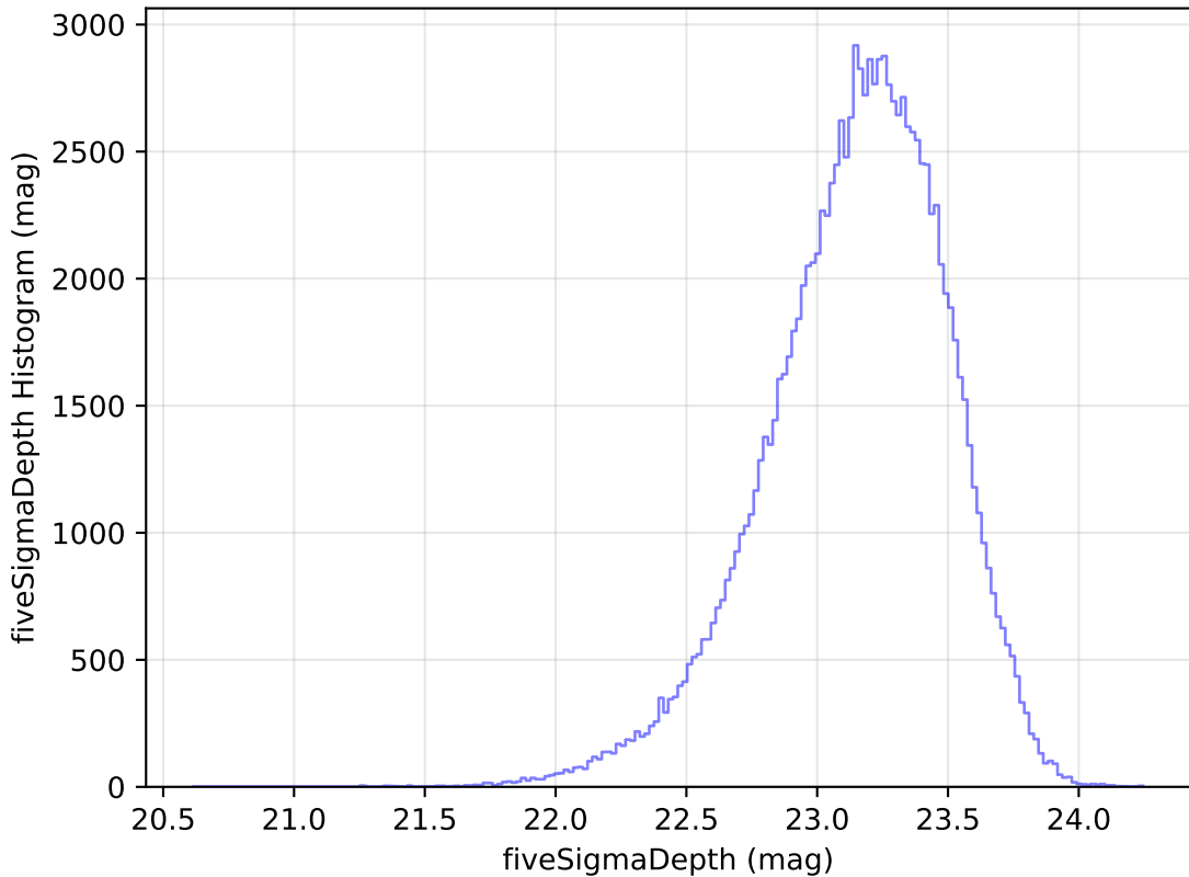
roll_pause_mjdp0_v3.4_10yrs All sky u band: fiveSigmaDepth Histogram
