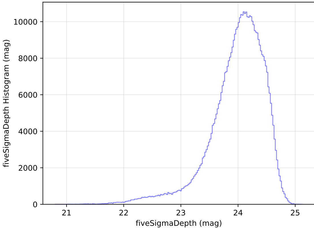
roll_pause_mjdp0_v3.4_10yrs All sky r band: fiveSigmaDepth Histogram
