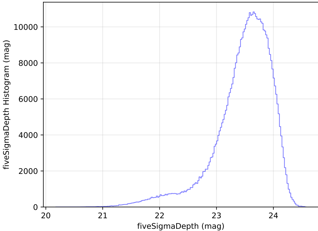
roll_pause_mjdp0_v3.4_10yrs All sky i band: fiveSigmaDepth Histogram
