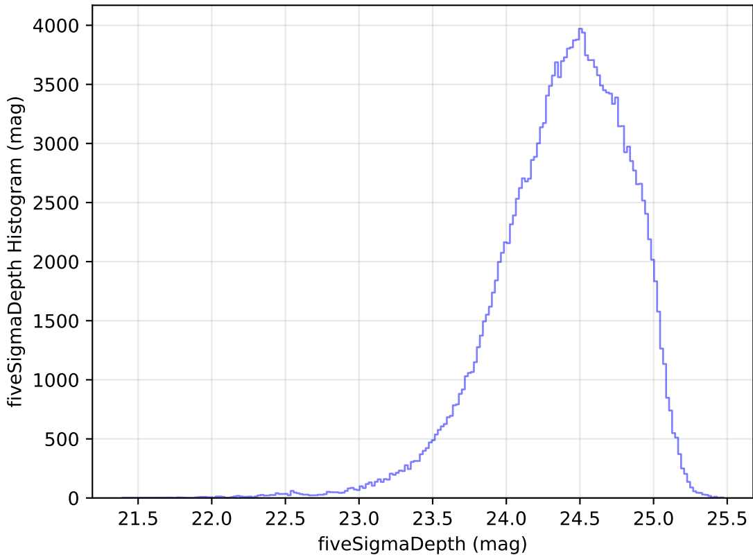
roll_pause_mjdp0_v3.4_10yrs All sky g band: fiveSigmaDepth Histogram
