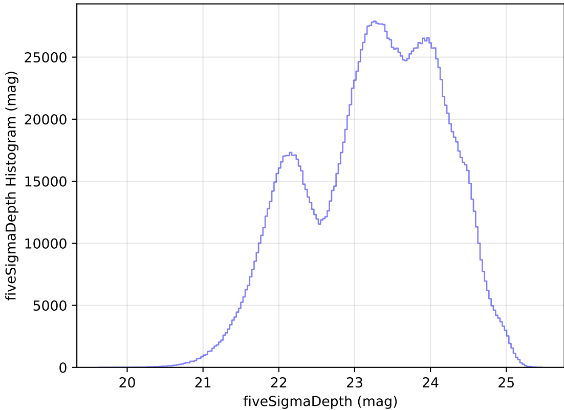
roll_pause_mjdp0_v3.4_10yrs All sky all bands: fiveSigmaDepth Histogram
