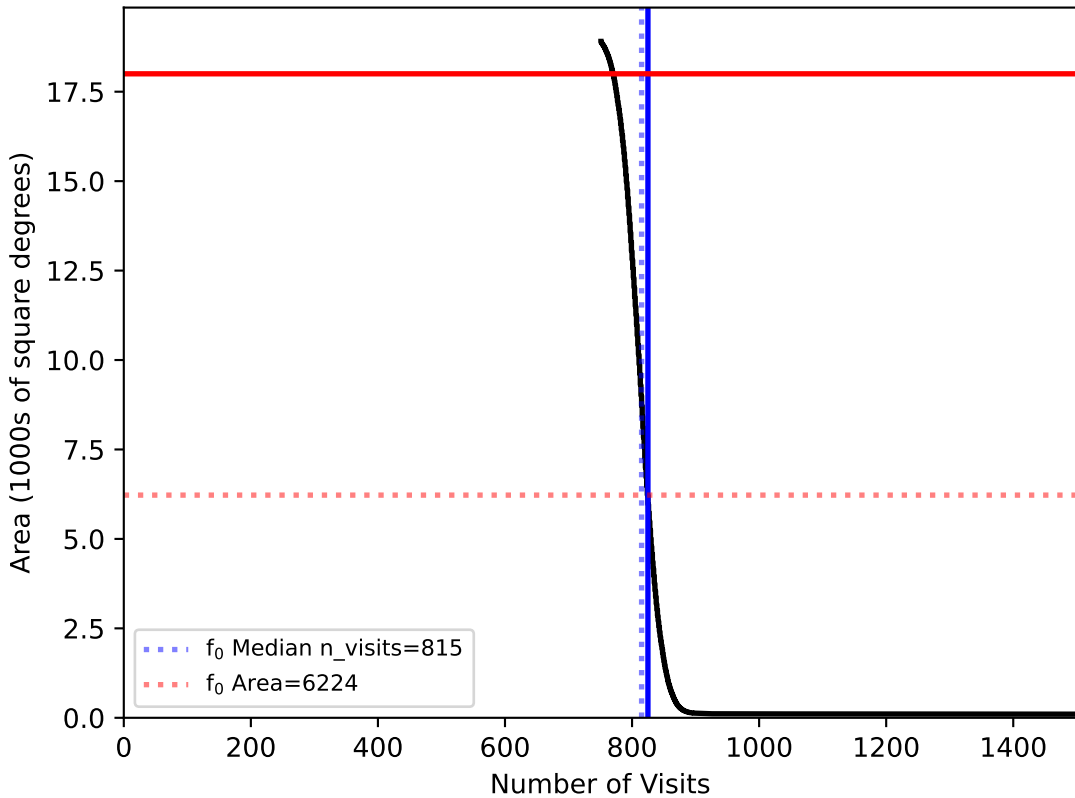
roll_pause_mjdp0_v3.4_10yrs WFD: fO
