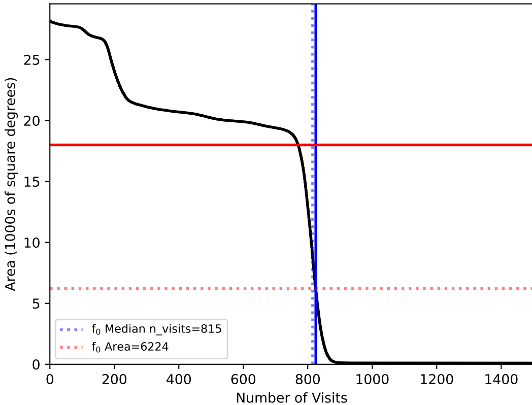
roll_pause_mjdp0_v3.4_10yrs All sky: f0
