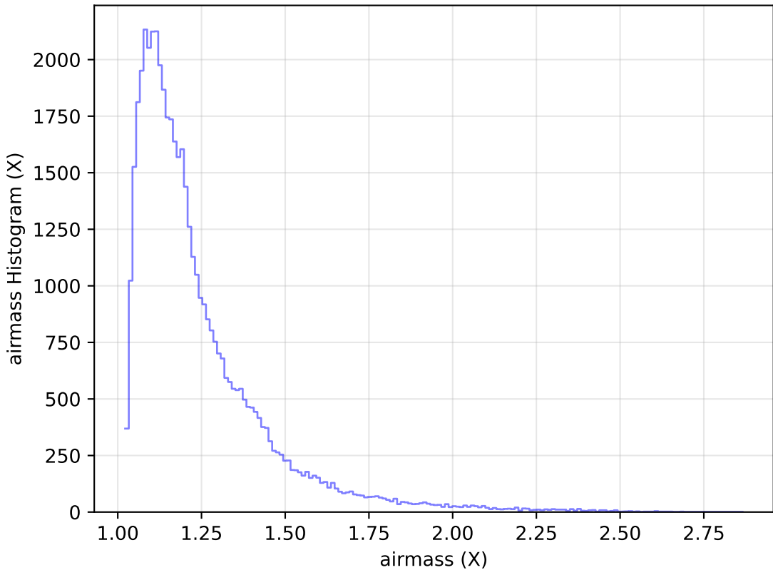
roll_pause_mjdp0_v3.4_10yrs Yr 1 y band: airmass Histogram
