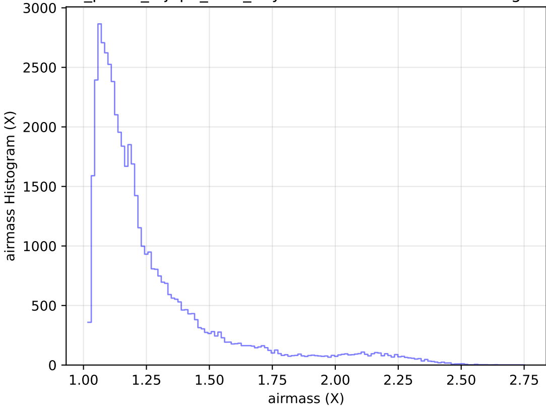
roll_pause_mjdp0_v3.4_10yrs Yr 1 r band: airmass Histogram
