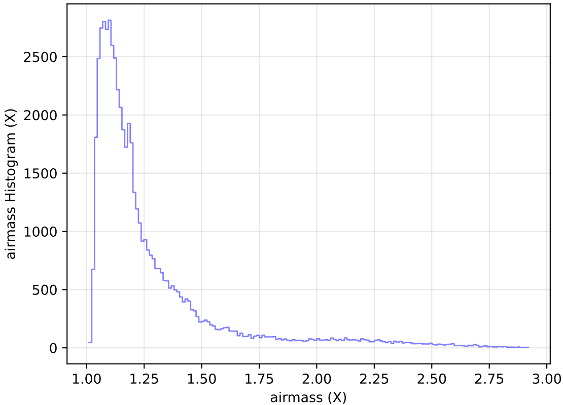
roll_pause_mjdp0_v3.4_10yrs Yr 1 i band: airmass Histogram
