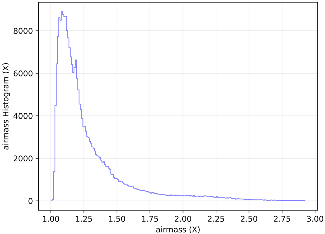
roll_pause_mjdp0_v3.4_10yrs Yr 1 all bands: airmass Histogram
