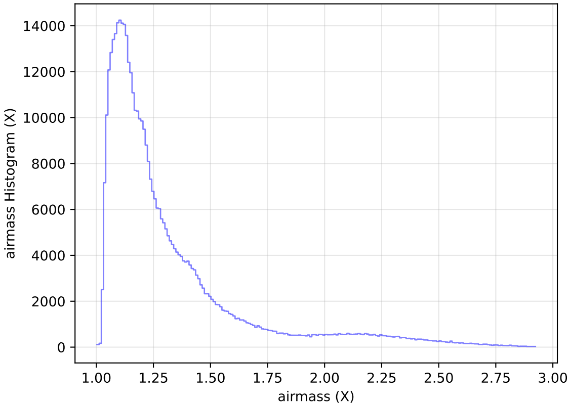
roll_pause_mjdp0_v3.4_10yrs WFD z band: airmass Histogram
