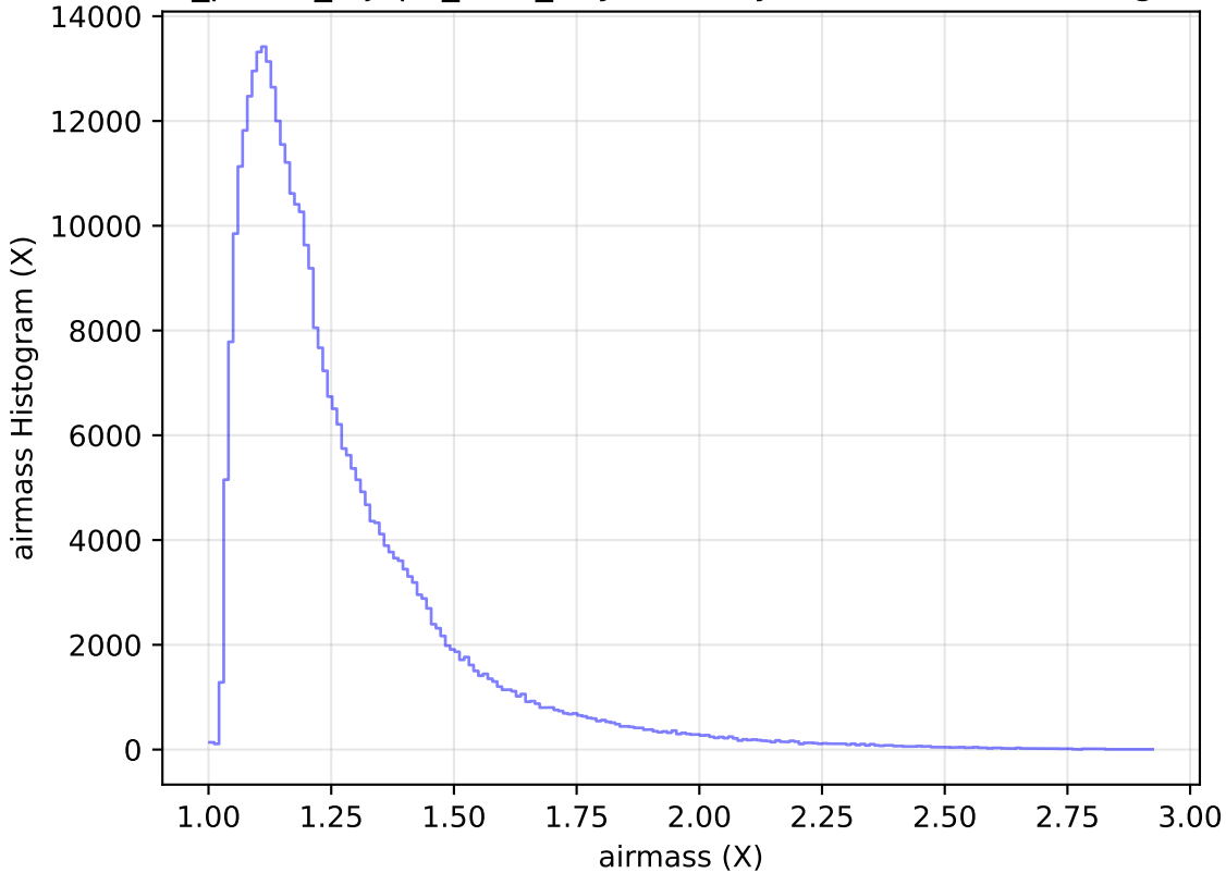
roll_pause_mjdp0_v3.4_10yrs WFD y band: airmass Histogram
