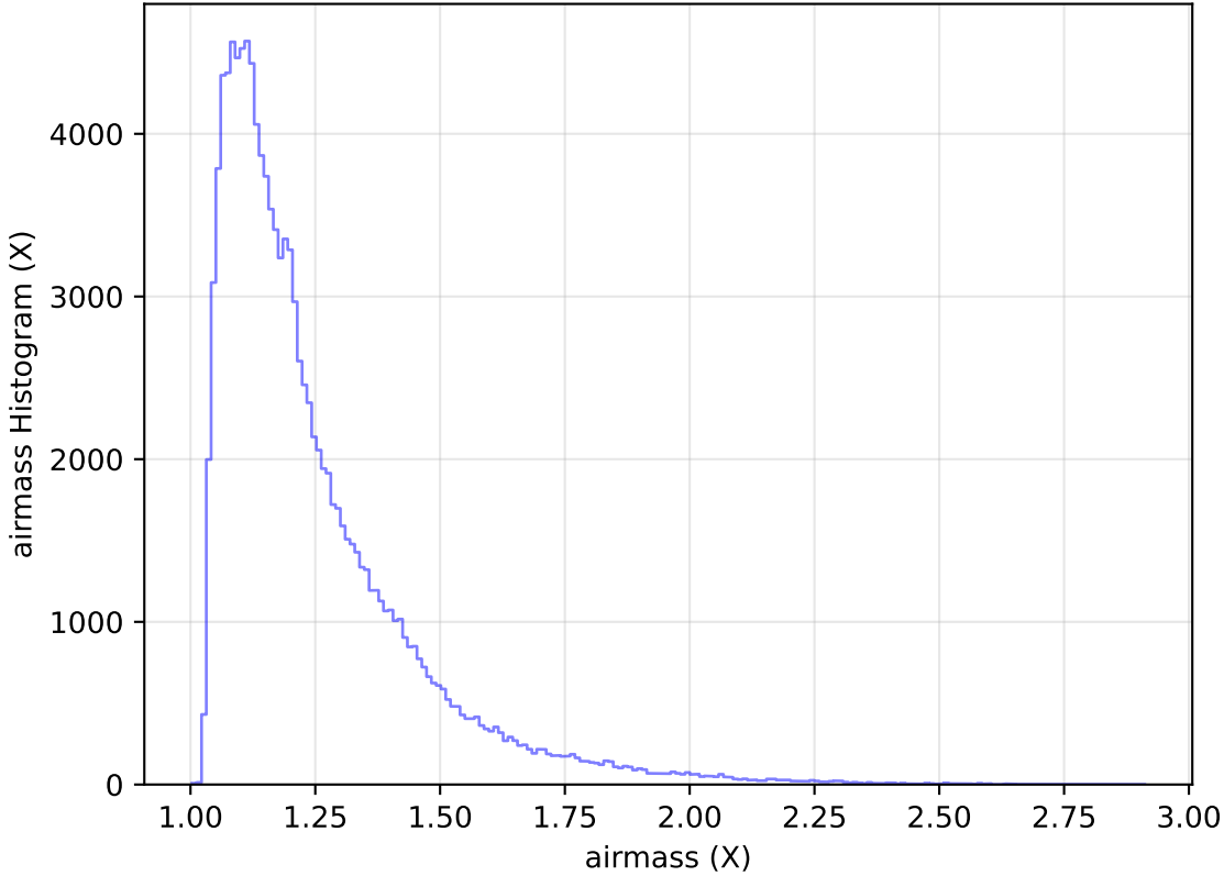
roll_pause_mjdp0_v3.4_10yrs WFD u band: airmass Histogram
