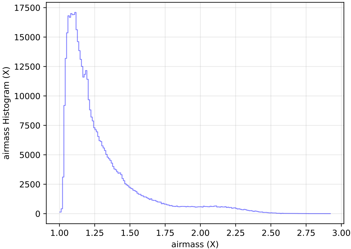
roll_pause_mjdp0_v3.4_10yrs WFD r band: airmass Histogram
