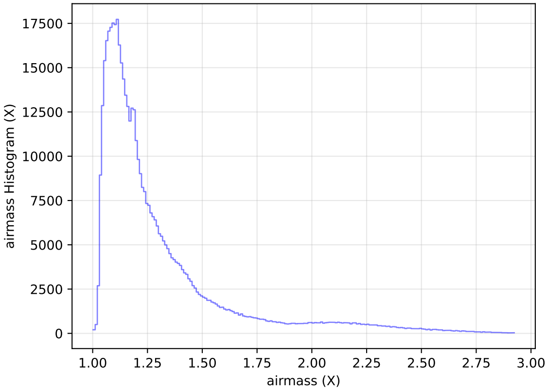
roll_pause_mjdp0_v3.4_10yrs WFD i band: airmass Histogram
