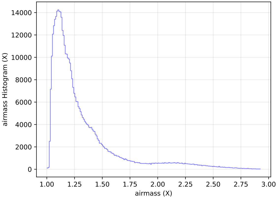
roll_pause_mjdp0_v3.4_10yrs All sky z band: airmass Histogram
