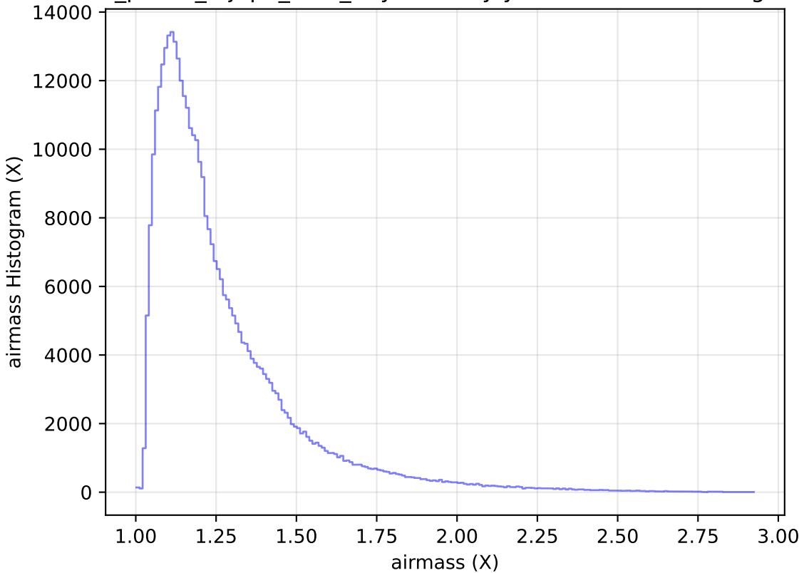
roll_pause_mjdp0_v3.4_10yrs All sky y band: airmass Histogram
