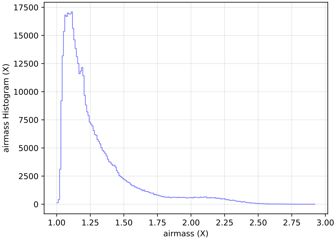
roll_pause_mjdp0_v3.4_10yrs All sky r band: airmass Histogram
