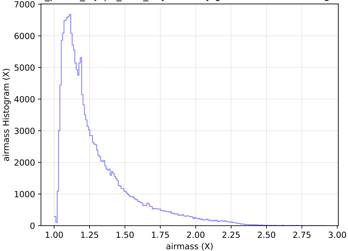
roll_pause_mjdp0_v3.4_10yrs All sky g band: airmass Histogram
