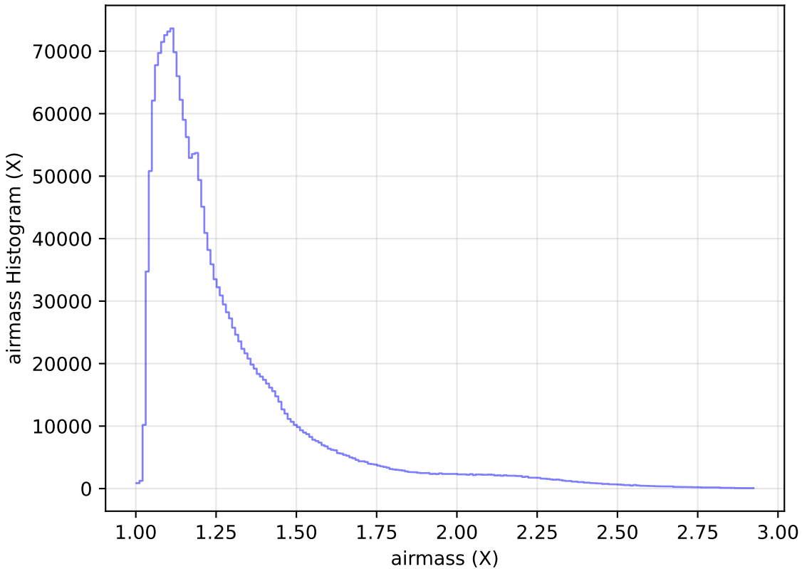
roll_pause_mjdp0_v3.4_10yrs All sky all bands: airmass Histogram
