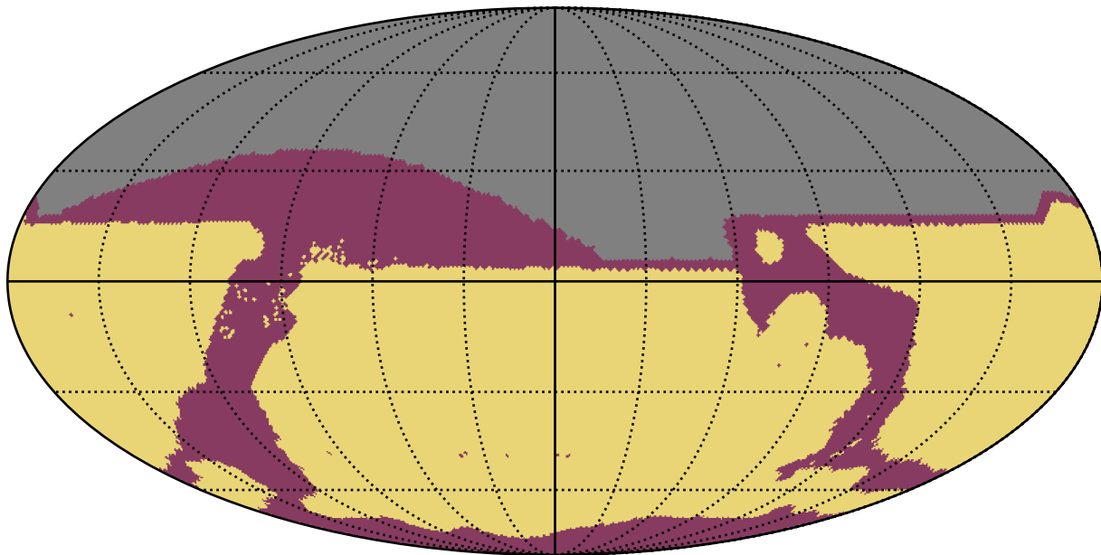
roll_pause_mjdp0_v3.4_10yrs All sky: RapidRevisits
