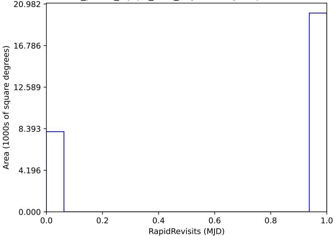
roll_pause_mjdp0_v3.4_10yrs All sky: RapidRevisits
