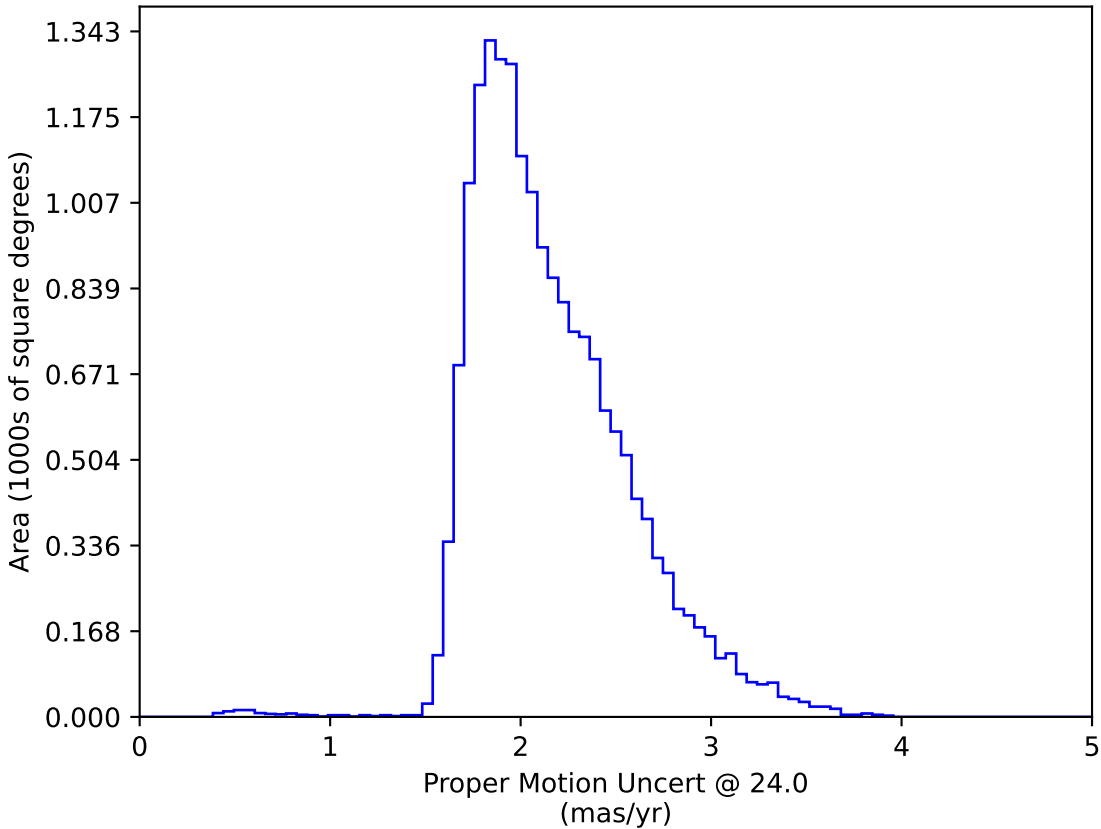
roll_pause_mjdp0_v3.4_10yrs WFD: Proper Motion Uncert @ 24.0
