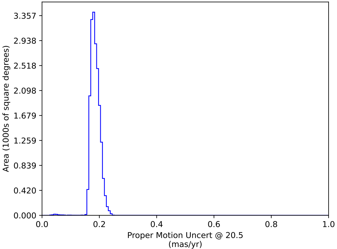
roll_pause_mjdp0_v3.4_10yrs WFD: Proper Motion Uncert @ 20.5
