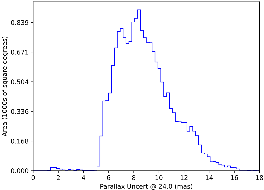
roll_pause_mjdp0_v3.4_10yrs WFD: Parallax Uncert @ 24.0
