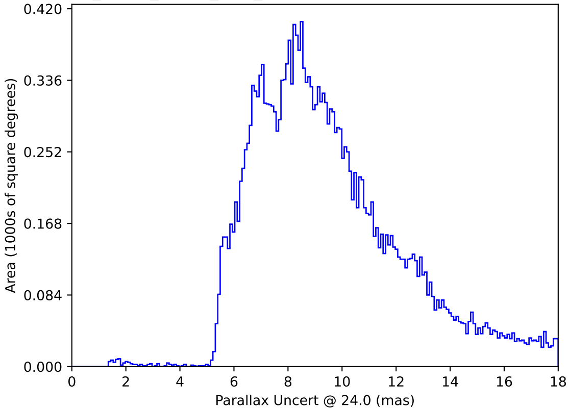
roll_pause_mjdp0_v3.4_10yrs All sky: Parallax Uncert @ 24.0
