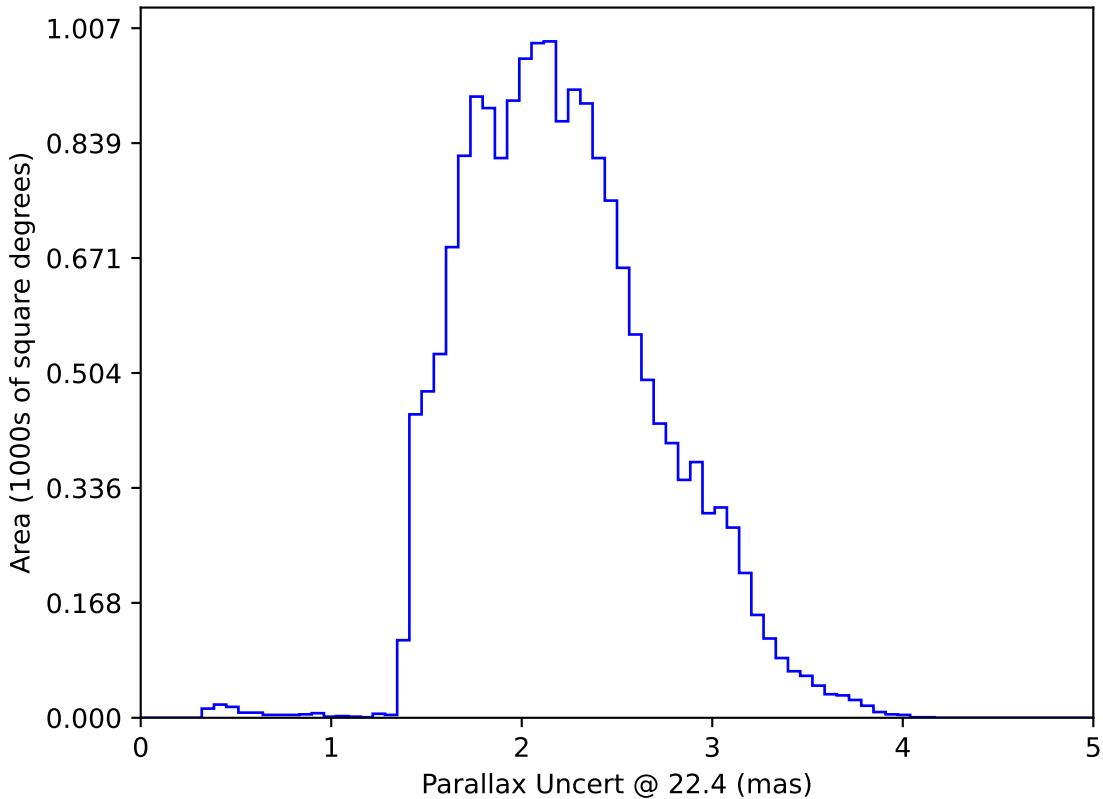
roll_pause_mjdp0_v3.4_10yrs WFD: Parallax Uncert @ 22.4
