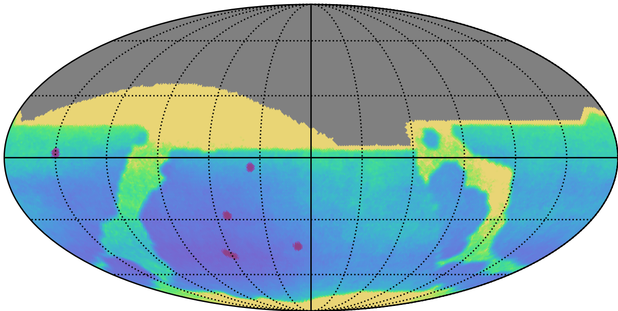
roll_pause_mjdp0_v3.4_10yrs All sky: Parallax Uncert @ 22.4
